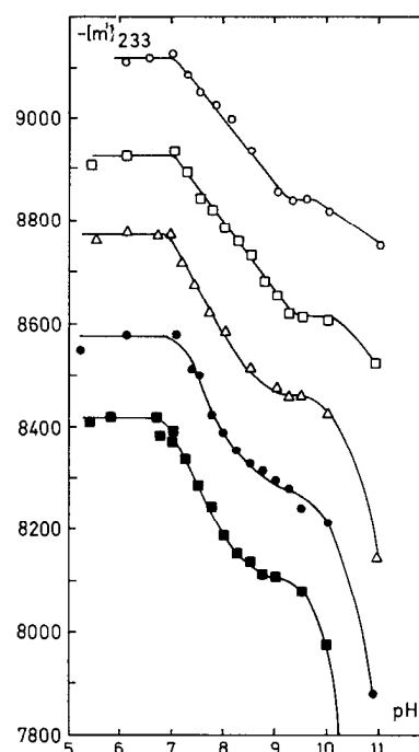
FIG. 1. The mean residue rotation at 233 nm of defatted HSA as a function of pH from 5.5 to 11 at the temperatures: \circ — \circ , 11^\circ ; \square — \square , 20^\circ ; \triangle — \triangle , 30^\circ ; \bullet — \bullet , 37.5^\circ ; \blacksquare — \blacksquare , 44^\circ . KCl, 0.2 M; protein concentration around 0.05%; 1 cm cell.
