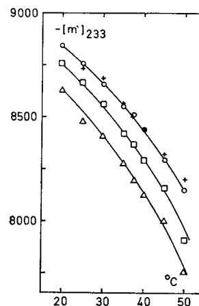
FIG. 2. The mean residue rotation at 233 nm of defatted HSA in variation of temperature at different pH values: +—+, pH 6.5; O—O, pH 7.0; □—□, pH 8.0; △—△, pH 9.0. KCl, 0.2 M; protein concentration around 0.05%; 1 cm cell. Each experimental point represents a separately prepared sample.
