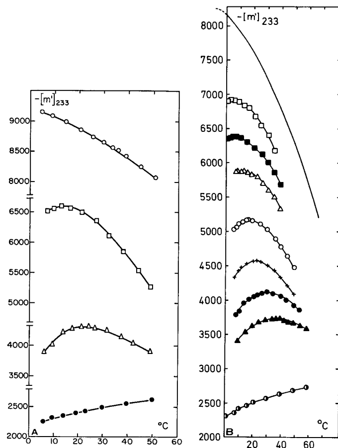
FIG. 7. The mean residue rotation at 233 nm of defatted HSA in variation of temperature at different concentrations of guanidine HCl; 0.2 M KCl; protein concentration around 0.4%; 1 mm cell. A, pH 7.5. Concentrations of guanidine HCl: ○—○, 0 M; □—□, 2 M; △—△, 3.5 M; ●—●, 8 M. B, pH 2.6. The unmarked line is in 0.2 M KCl, data from Fig. 5, concentrations of guanidine HCl: □—□, 2 M; ■—■, 2.5 M; △—△, 3 M; ○—○, 3.5 M; ×—×, 4 M; ●—●, 4.5 M; ▲—▲, 5 M; ●—●, 8 M. The measurement for each molarity of guanidine HCl and pH is made on the same sample, with control for reversibility after the experiment. The (m')_{233} measured in 8 M guanidine HCl at various temperatures of this figure and Fig. 6 are used as the rotation of complete unfolded HSA in calculating the helix contents of Table II.
