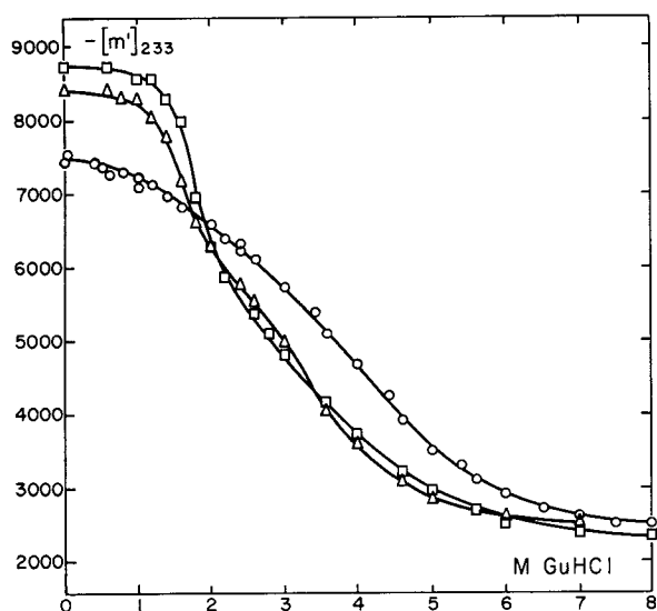
FIG. 6. The mean residue rotation at 233 nm of defatted HSA at different concentrations of guanidine HCl: at pH 9.2, △—△; at pH 5.5, □—□; at pH 2.6, ○—○. KCl, 0.2 M; protein concentration around 0.4%; 1 cm cell; temperature, 23°.
