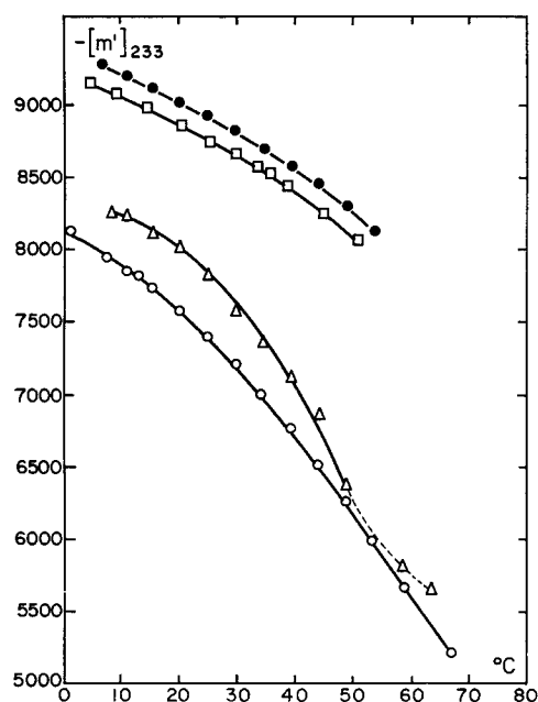
FIG. 5. The mean residue rotation at 233 nm of defatted HSA in variation of temperature at different pH. ●—●, pH 5.5; □—□, pH 7.5; △—△, pH 4.0; ○—○, pH 2.6. KCl, 0.2 M; protein concentration around 0.05%; 1 cm cell.
