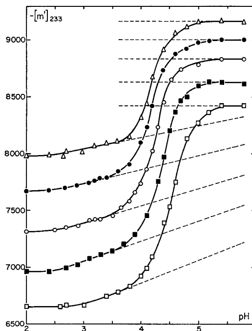
FIG. 3. The mean residue rotation at 233 nm ( m'_{233} ) of defatted HSA as a function of pH from 5.5 to 2.0 at the temperatures: △—△, 11°; ●—●, 20°; ○—○, 30°; ■—■, 37.5°; □—□, 44°. KCl, 0.2 M; protein concentration around 0.05%; 1 cm cell. The broken lines are extrapolations of the folded (N form) and the partly unfolded (F form) to constitute the rotations of the respective forms in the transition region in calculating the apparent equilibrium constant for the N-F transformation.
