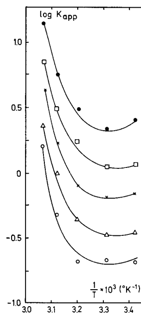
FIG. 4. Van't Hoff plots for the N-F transition of defatted HSA from the data of Fig. 3. ●—●, pH 4.1; □—□, pH 4.2; △—△, pH 4.4; ○—○, pH 4.5. The curve (×—×) is the average of the \log K_{app} at the quoted pH and constitute the basis for the calculation of the enthalpies listed in Table I.
